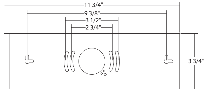
Mounting back plate
